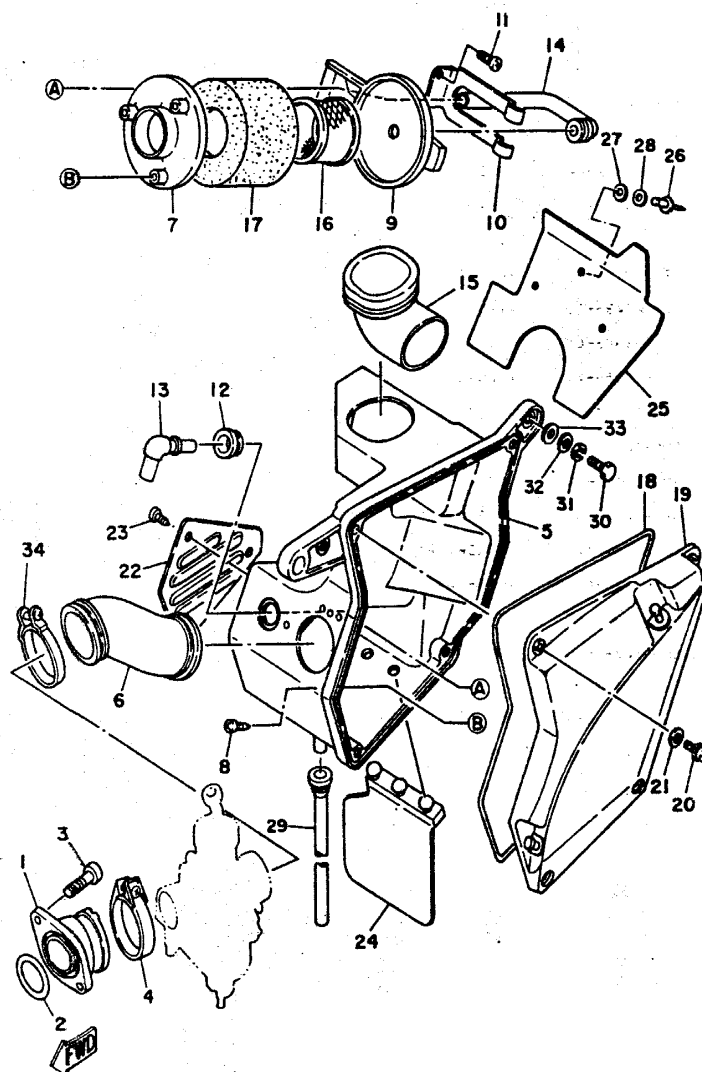
FIG. 7 INTAKE
